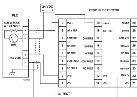
Figure 12—X3301 Detector Wired for Isolated 0 to 20 mA Current Output (Sourcing)
