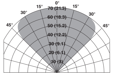
Field of View at Indicated Distance in Feet (m) for Methane at Medium Sensitivity (32 inch plume)
